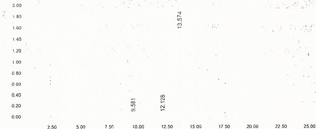
Auto-Scaled Chromatogram
